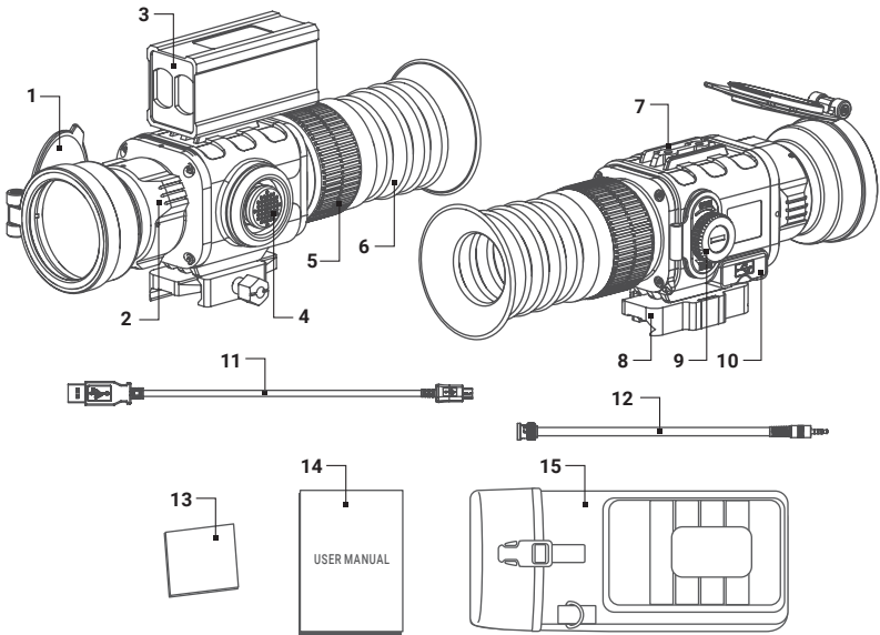
FIGURE 1-1. PYTHON-MICRO TS50 MAIN PARTS AND COMPONENTS TABLE 1-1. PYTHON-MICRO MAIN PARTS AND COMPONENTS
